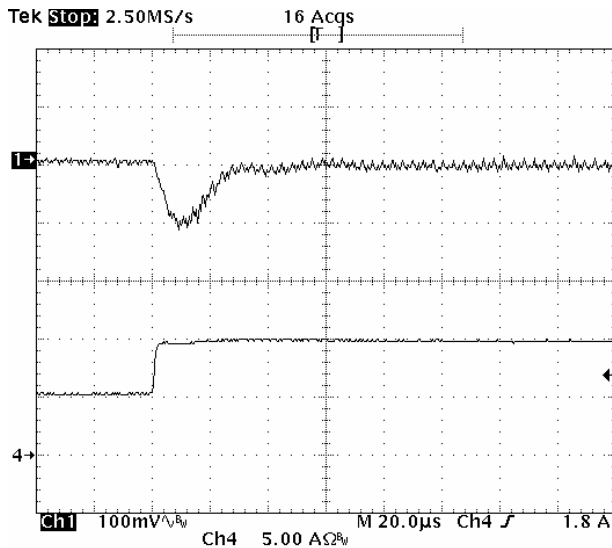
Fig-1.5V-6: Output voltage response for V_{out}=1.5V to positive load current step-change from 5A to 10A with slew rate of 5A/\mu s at V_{in}=5.0V . C_o=47\mu F \times 4 ceramic + 1\mu F ceramic. Top trace: output voltage (100mV/div.) Bottom trace: load current (5A/div.) Time scale: 20µs/div.
