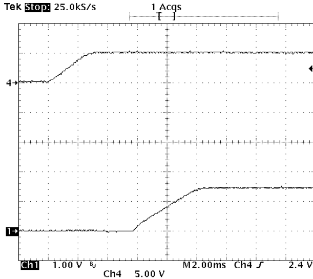
Fig-1.5V-4: Turn-on transient for V_{out}=1.5V with application of V_{in} at full rated load current (resistive) and 47\mu F \times 4 external capacitance at V_{in}=5.0V . Top trace: V_{in} (5V/div.) Bottom trace: output voltage (1V/div.) Time scale: 2ms/div.
