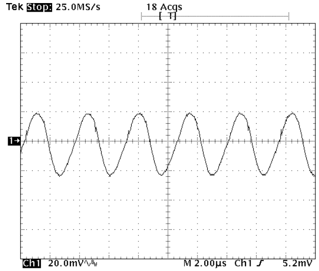
Fig-1.5V-5: Output voltage ripple (20mV/div.) for V_{out}=1.5V at full rated load current into a resistive load with external capacitance 47\mu F \times 4 ceramic + 1\mu F ceramic at V_{in}=5.0V . Time scale: 2µs/div
