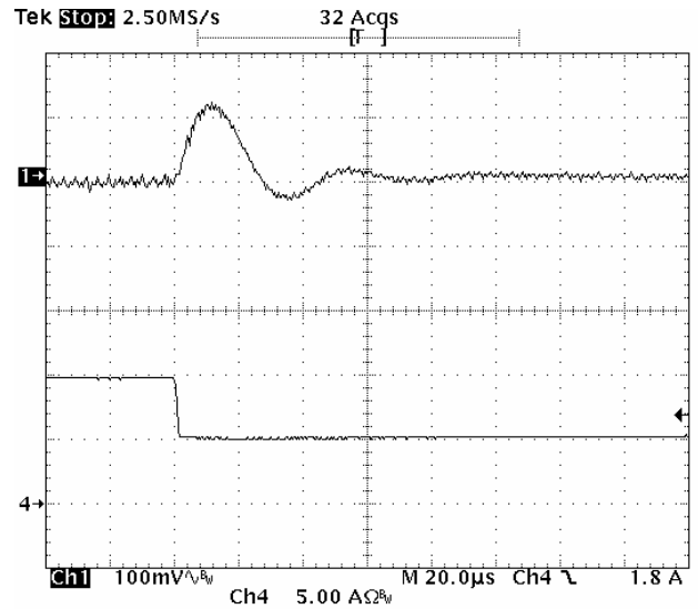
Fig-1.5V-7: Output voltage response for V_{out}=1.5V to positive load current step-change from 10A to 5A with slew rate of -5A/\mu s at V_{in}=5.0V . C_o=47\mu F \times 4 ceramic + 1\mu F ceramic. Top trace: output voltage (100mV/div.) Bottom trace: load current (5A/div.) Time scale: 20µs/div.
