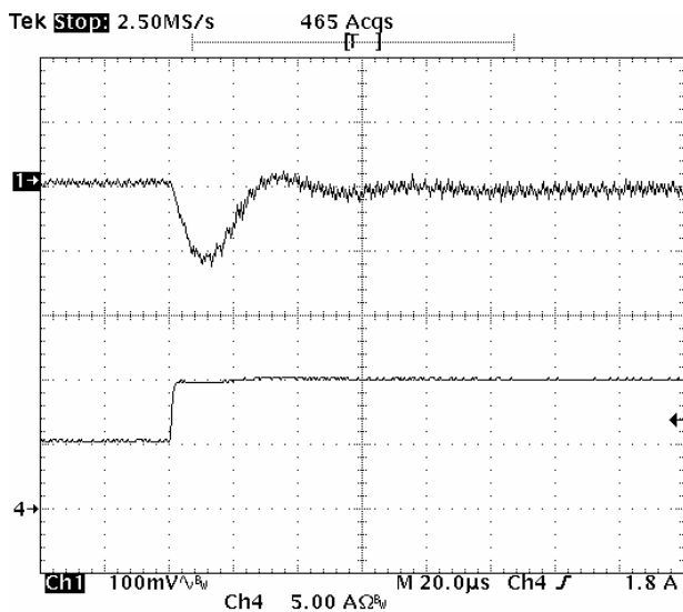
Fig-1.8V-6: Output voltage response for V_{out}=1.8V to positive load current step-change from 5A to 10A with slew rate of 5A/\mu s at V_{in}=5.0V . C_o=47\mu F \times 4 ceramic + 1\mu F ceramic. Top trace: output voltage (100mV/div.) Bottom trace: load current (5A/div.) Time scale: 20µs/div.
