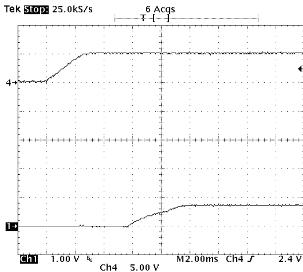
Fig-0.7525V-4: Turn-on transient for V_{out}=0.7525V with application of V_{in} at full rated load current (resistive) and 47\mu F \times 4 external capacitance at V_{in}=5.0V . Top trace: V_{in} (5V/div.) Bottom trace: output voltage (1V/div.) Time scale: 2ms/div.
