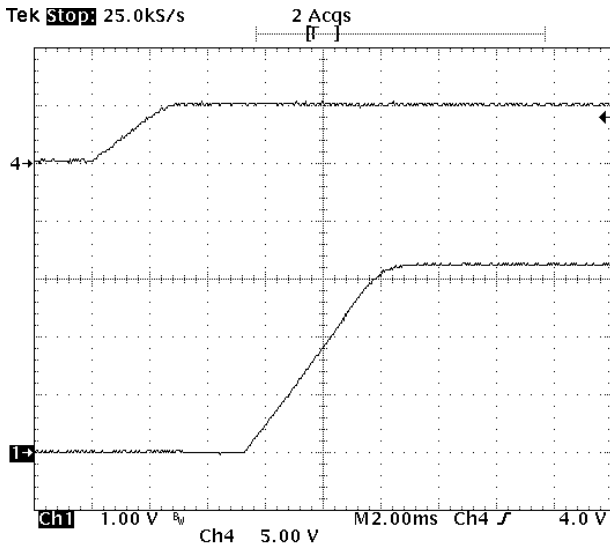
Fig-3.3V-4: Turn-on transient for V_{out}=3.3V with application of V_{in} at full rated load current (resistive) and 47\mu F \times 4 external capacitance at V_{in}=5.0V . Top trace: V_{in} (5V/div.) Bottom trace: output voltage (1V/div.) Time scale: 2ms/div.
