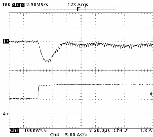
Fig-2.5V-6: Output voltage response for V_{out}=2.5V to positive load current step-change from 5A to 10A with slew rate of 5A/\mu s at V_{in}=5.0V . C_o=47\mu F \times 4 ceramic + 1µF ceramic. Top trace: output voltage (100mV/div.) Bottom trace: load current (5A/div.) Time scale: 20µs/div.
