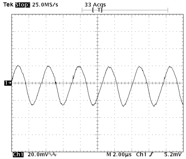
Fig-1.8V-5: Output voltage ripple (20mV/div.) for V_{out}=1.8V at full rated load current into a resistive load with external capacitance 47\mu F \times 4 ceramic + 1\mu F ceramic at V_{in}=5.0V . Time scale: 2µs/div
