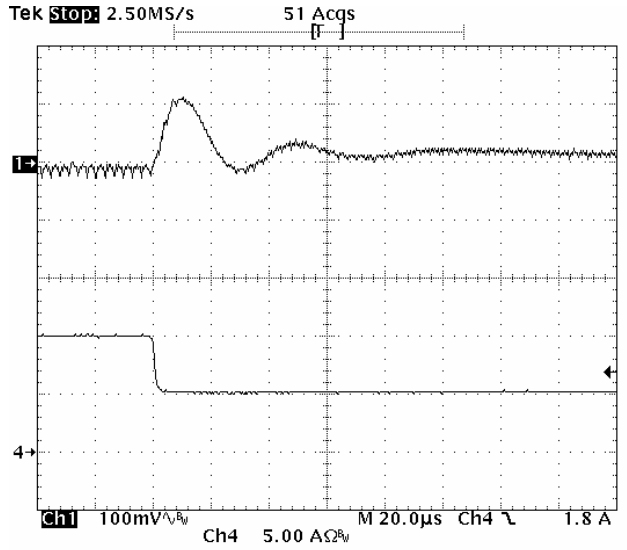
Fig-2.5V-7: Output voltage response for V_{out}=2.5V to positive load current step-change from 10A to 5A with slew rate of -5A/\mu s at V_{in}=5.0V . C_o=47\mu F \times 4 ceramic + 1µF ceramic. Top trace: output voltage (100mV/div.) Bottom trace: load current (5A/div.) Time scale: 20µs/div.
