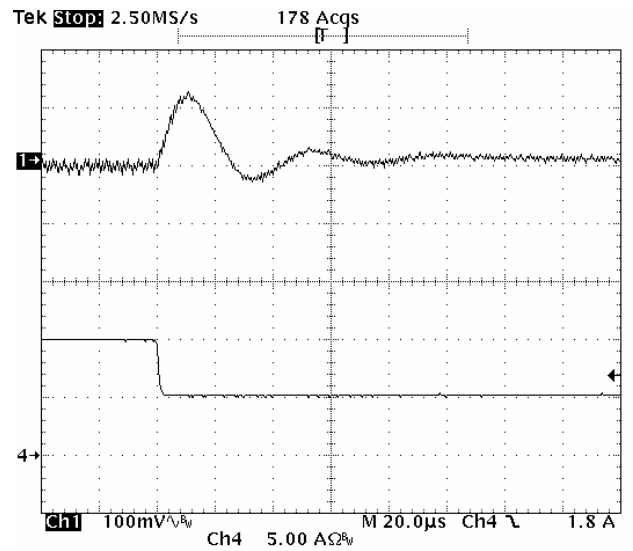
Fig-1.8V-7: Output voltage response for V_{out}=1.8V to positive load current step-change from 10A to 5A with slew rate of -5A/\mu s at V_{in}=5.0V . C_o=47\mu F \times 4 ceramic + 1\mu F ceramic. Top trace: output voltage (100mV/div.) Bottom trace: load current (5A/div.) Time scale: 20µs/div.
