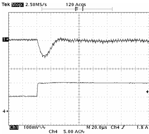
Fig-2.0V-6: Output voltage response for V_{out}=2.0V to positive load current step-change from 5A to 10A with slew rate of 5A/\mu s at V_{in}=5.0V . C_o=47\mu F \times 4 ceramic + 1μF ceramic.
