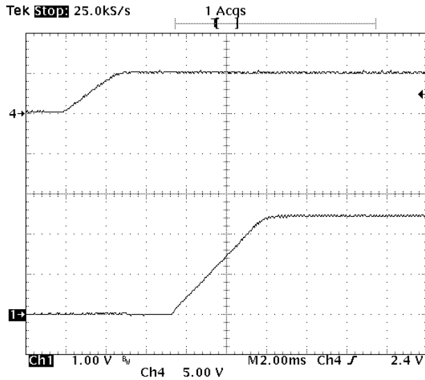
Fig-2.5V-4: Turn-on transient for V_{out}=2.5V with application of V_{in} at full rated load current (resistive) and 47\mu F \times 4 external capacitance at V_{in}=5.0V . Top trace: V_{in} (5V/div.) Bottom trace: output voltage (1V/div.) Time scale: 2ms/div.
