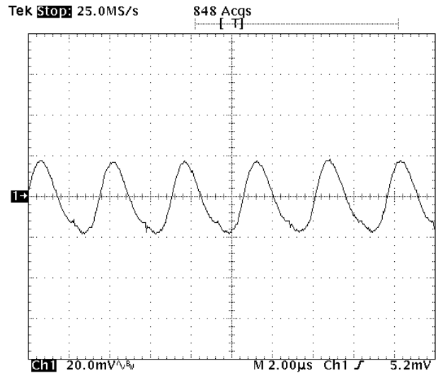
Fig-3.3V-5: Output voltage ripple (20mV/div.) for V_{out}=3.3V at full rated load current into a resistive load with external capacitance 47\mu F \times 4 ceramic + 1\mu F ceramic at V_{in}=5.0V . Time scale: 2µs/div
