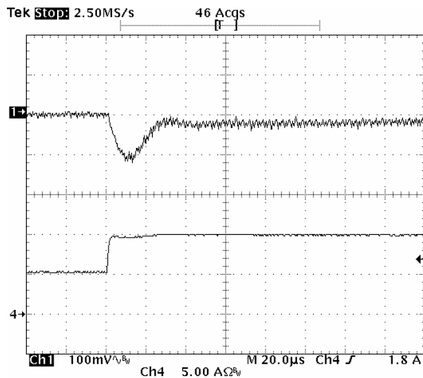
Fig-1.2V-6: Output voltage response for V_{out}=1.2V to positive load current step-change from 5A to 10A with slew rate of 5A/\mu s at V_{in}=5.0V . C_o=47\mu F \times 4 ceramic + 1\mu F ceramic. Top trace: output voltage (100mV/div.) Bottom trace: load current (5A/div.) Time scale: 20\mu s /div.
