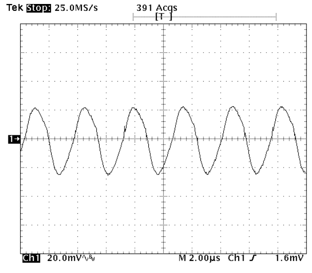
Fig-2.0V-5: Output voltage ripple (20mV/div.) for V_{out}=2.0V at full rated load current into a resistive load with external capacitance 47\mu F \times 4 ceramic + 1μF ceramic at V_{in}=5.0V .
