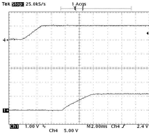
Fig-1.2V-4: Turn-on transient for V_{out}=1.2V with application of V_{in} at full rated load current (resistive) and 47\mu F \times 4 external capacitance at V_{in}=5.0V . Top trace: V_{in} (5V/div.) Bottom trace: output voltage (1V/div.) Time scale: 2ms/div.
