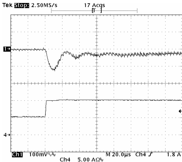
Fig-3.3V-6: Output voltage response for V_{out}=3.3V to positive load current step-change from 5A to 10A with slew rate of 5A/\mu s at V_{in}=5.0V . C_o=47\mu F \times 4 ceramic + 1\mu F ceramic. Top trace: output voltage (100mV/div.) Bottom trace: load current (5A/div.) Time scale: 20µs/div.
