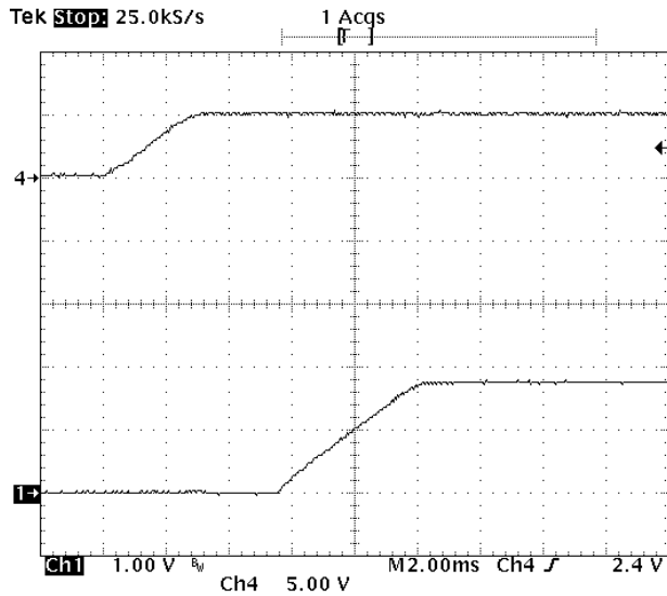
Fig-1.8V-4: Turn-on transient for V_{out}=1.8V with application of V_{in} at full rated load current (resistive) and 47\mu F \times 4 external capacitance at V_{in}=5.0V . Top trace: V_{in} (5V/div.) Bottom trace: output voltage (1V/div.) Time scale: 2ms/div.
