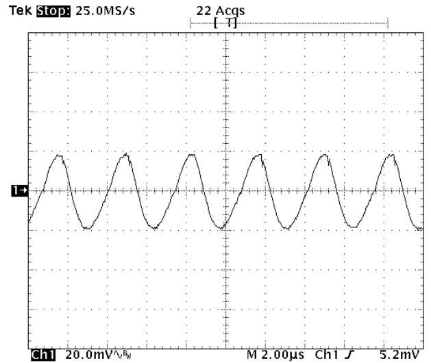
Fig-1.2V-5: Output voltage ripple (20mV/div.) for V_{out}=1.2V at full rated load current into a resistive load with external capacitance 47\mu F \times 4 ceramic + 1\mu F ceramic at V_{in}=5.0V . Time scale: 2\mu s /div
