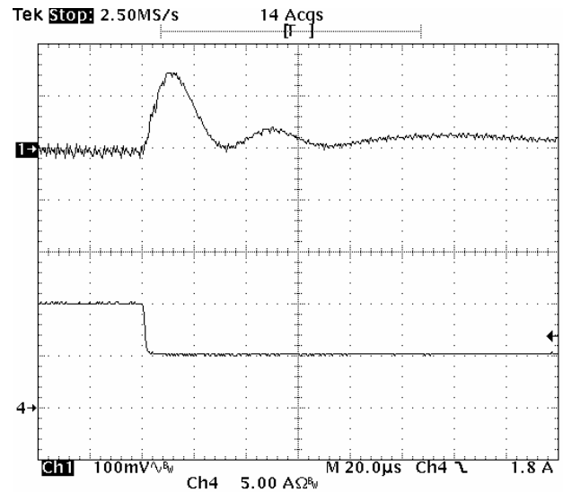
Fig-3.3V-7: Output voltage response for V_{out}=3.3V to positive load current step-change from 10A to 5A with slew rate of -5A/\mu s at V_{in}=5.0V . C_o=47\mu F \times 4 ceramic + 1\mu F ceramic. Top trace: output voltage (100mV/div.) Bottom trace: load current (5A/div.) Time scale: 20µs/div.
