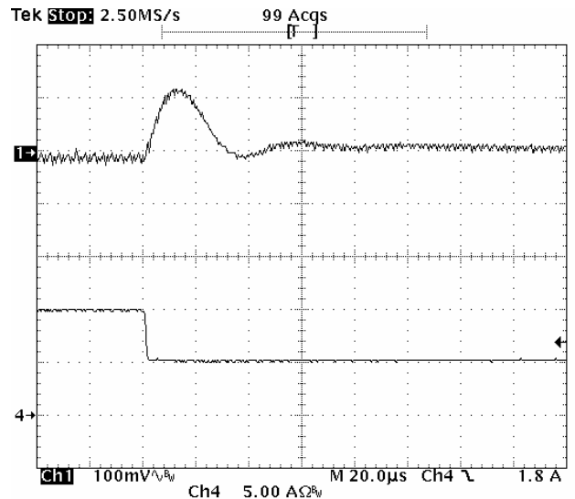
Fig-1.2V-7: Output voltage response for V_{out}=1.2V to positive load current step-change from 10A to 5A with slew rate of -5A/\mu s at V_{in}=5.0V . C_o=47\mu F \times 4 ceramic + 1\mu F ceramic. Top trace: output voltage (100mV/div.) Bottom trace: load current (5A/div.) Time scale: 20\mu s /div.
