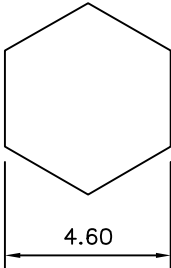
RECOMMENDED CRIMP SLEEVE A/F HEX
