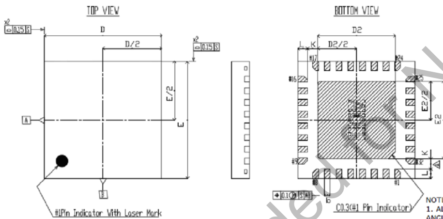
32-Lead QFN 5x 5mm
