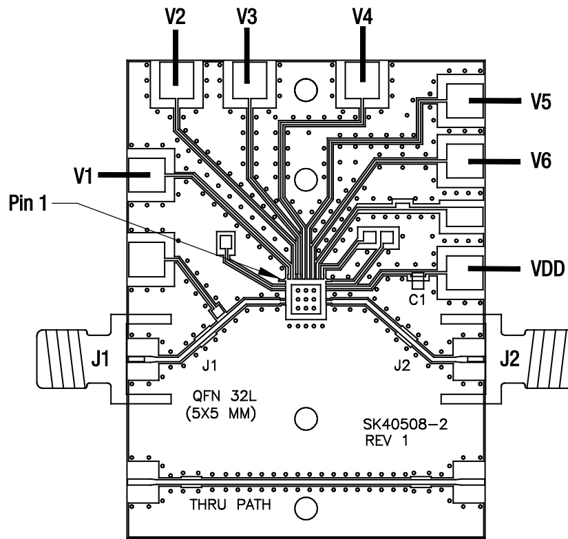
Figure 8. Evaluation Board Assembly Diagram
