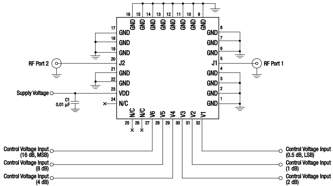
Figure 7. SKY12353-470LF Evaluation Board Schematic Diagram
