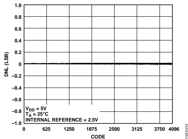
Figure 12. Differential Nonlinearity (DNL) vs. Code
