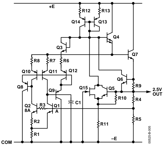
Figure 5. Schematic Diagram
