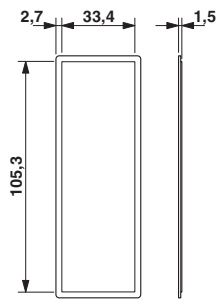
Dimensional drawing
