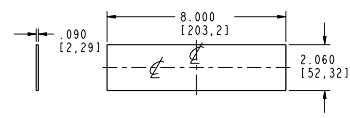
PANEL SIZE
