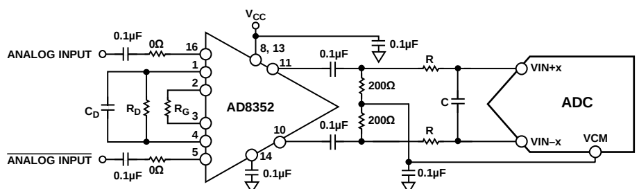
Figure 43. Differential Input Configuration Using the AD8352
