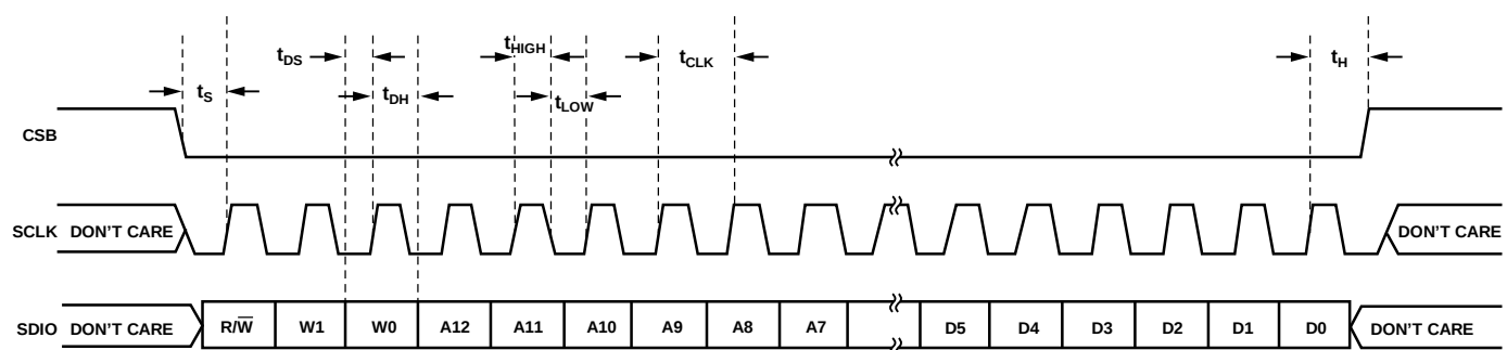
Figure 59. Serial Port Interface Timing Diagram
