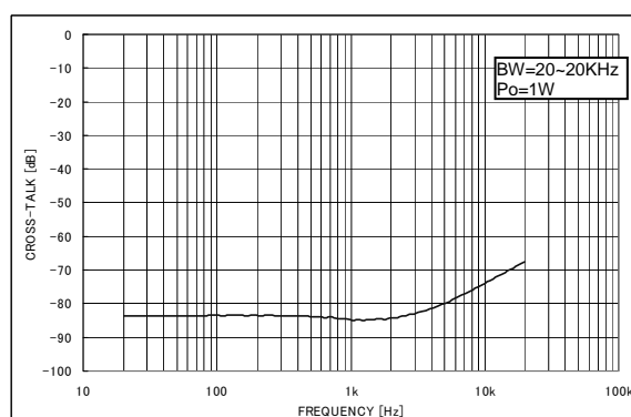
Fig.18 Crosstalk - Frequency
