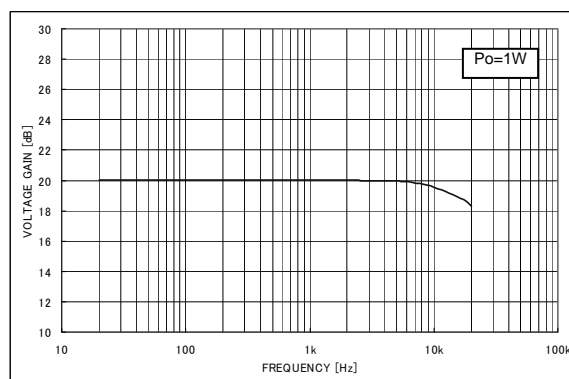
Fig.14 Voltage gain - Frequency
