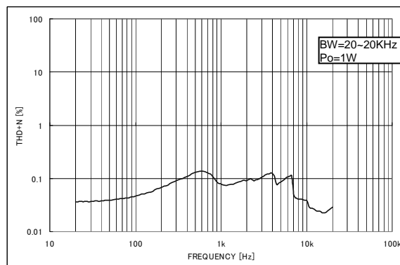
Fig.16 THD+N - Frequency
