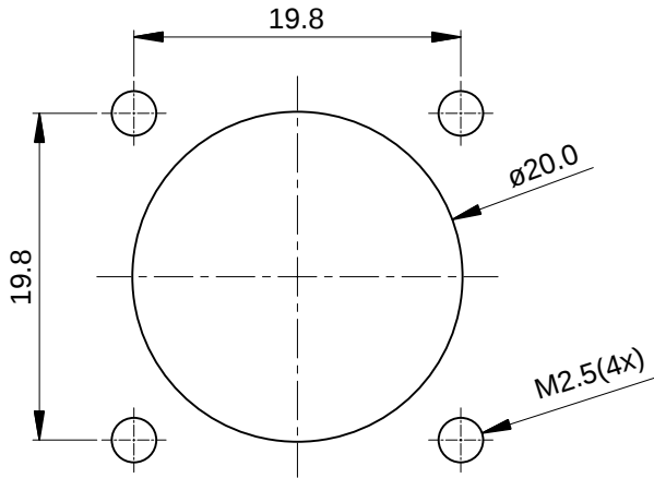
MOUNTING HOLE
