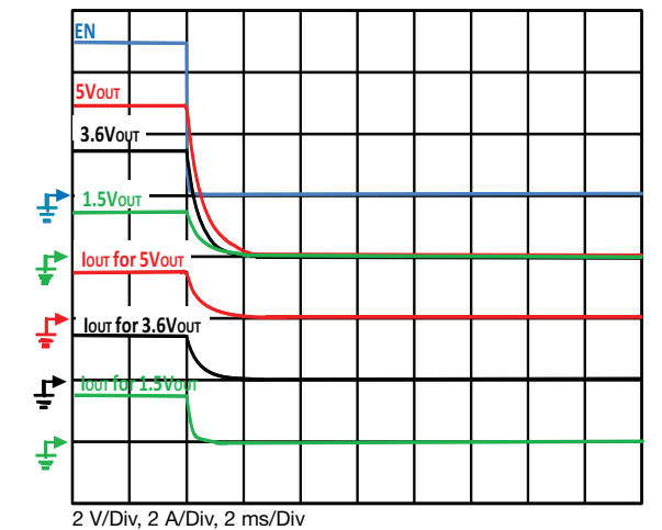
Figure 26 - Typical Fall Time C_{OUT} = 200 \mu F , C_{IN} = 4.7 \mu F , I_{OUT} = 1.5 A
