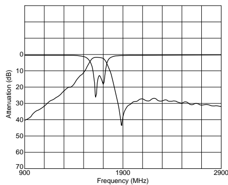
Frequency Characteristics
