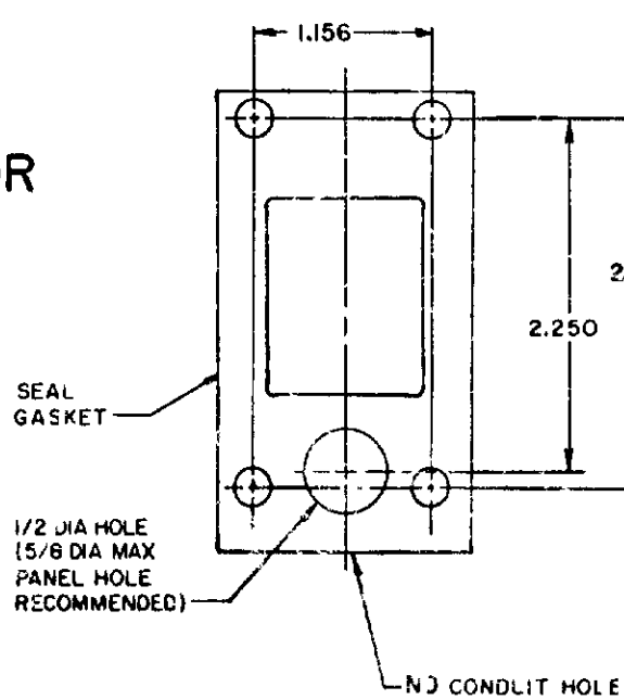
CABLE EXTENSION TYPE 7N ACTUATOR
