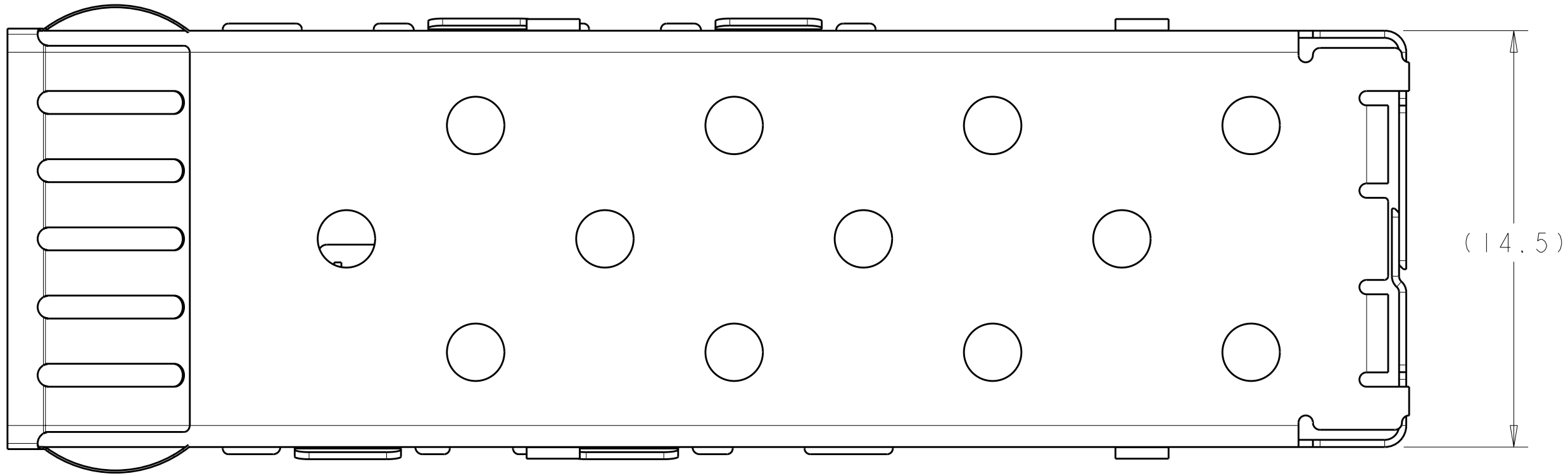
2007198-1 TOP VIEW
