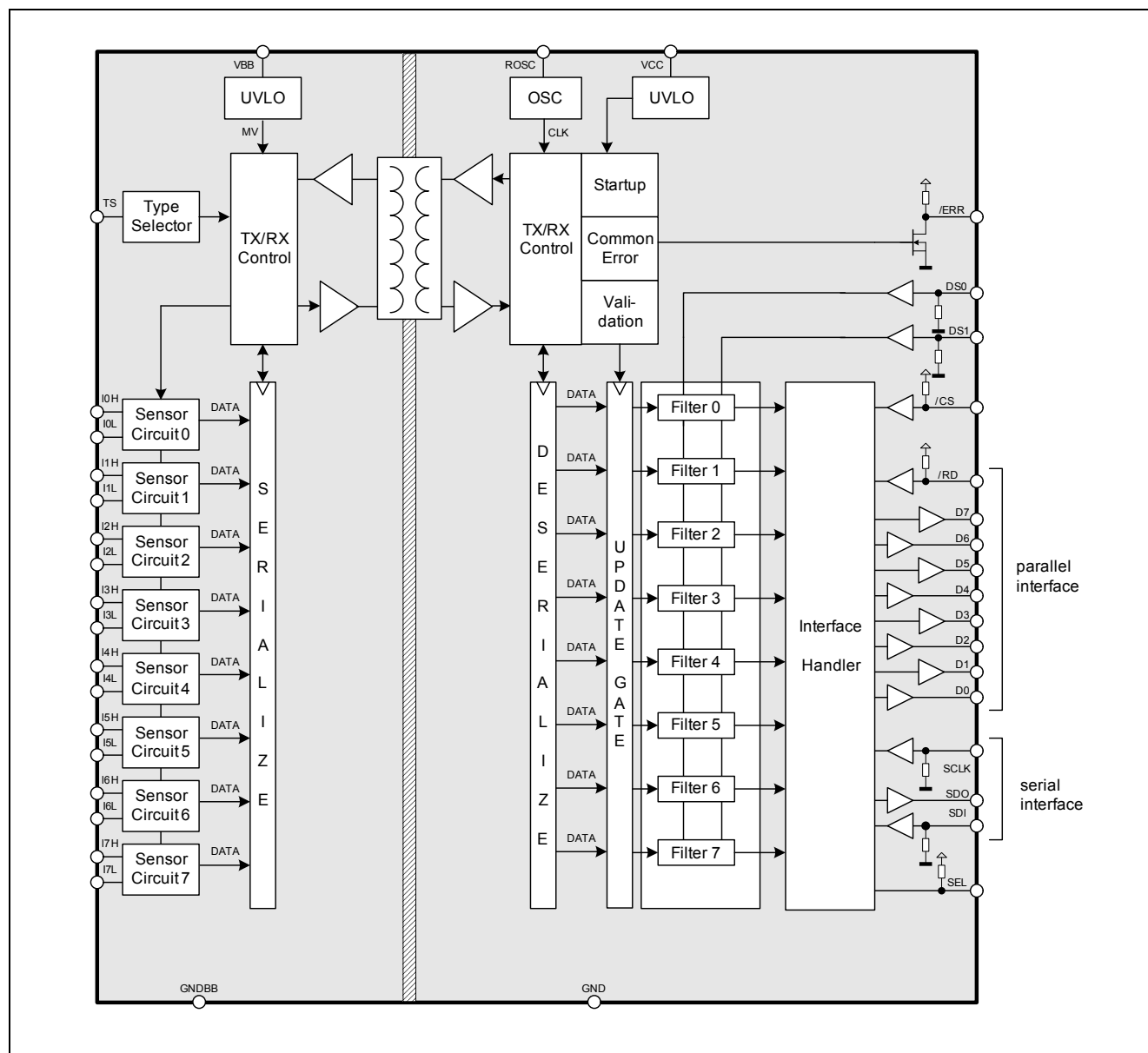
Figure 2 Block Diagram
