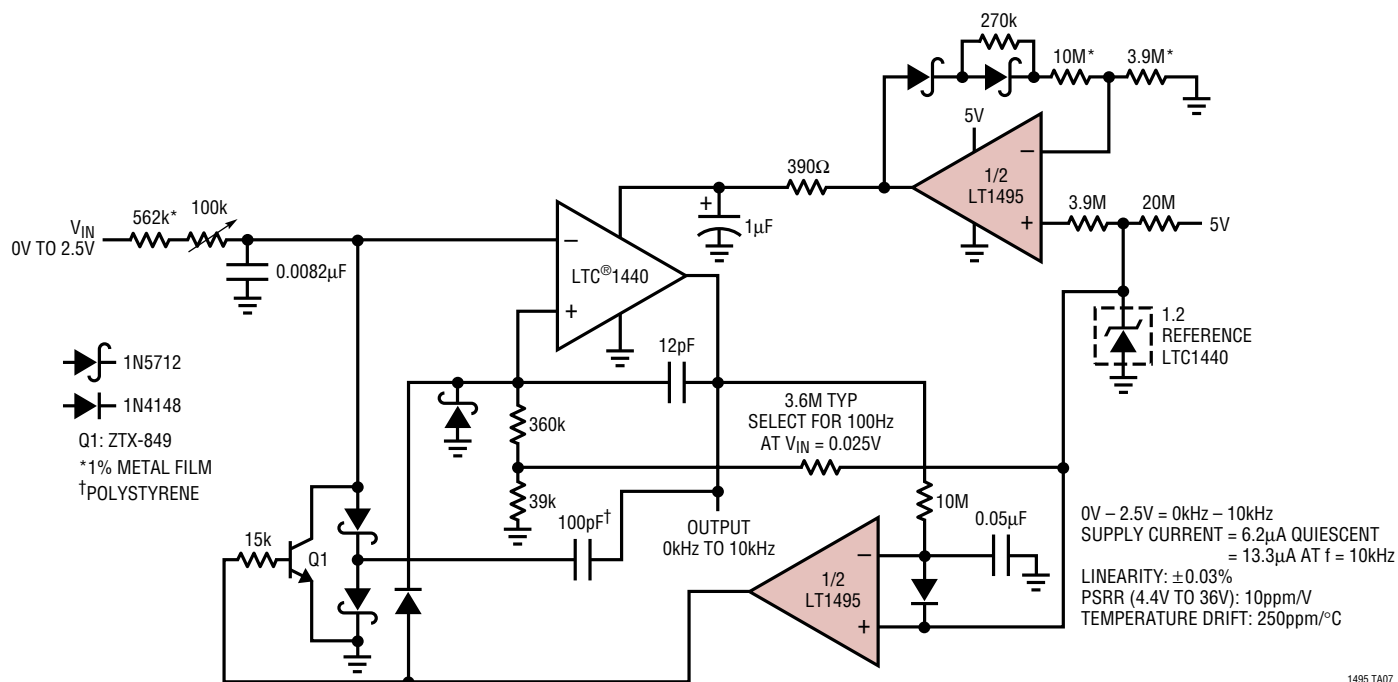
13μA, 0kHz to 10kHz Voltage to Frequency Converter
