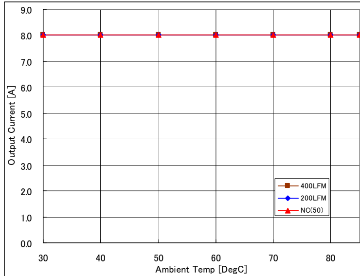
Fig 5.0V-1: Available load current vs. ambient temperature and airflow rates for Vout=5.0V with Vin=12V. Maximum component temperature ≤ 120°C.
