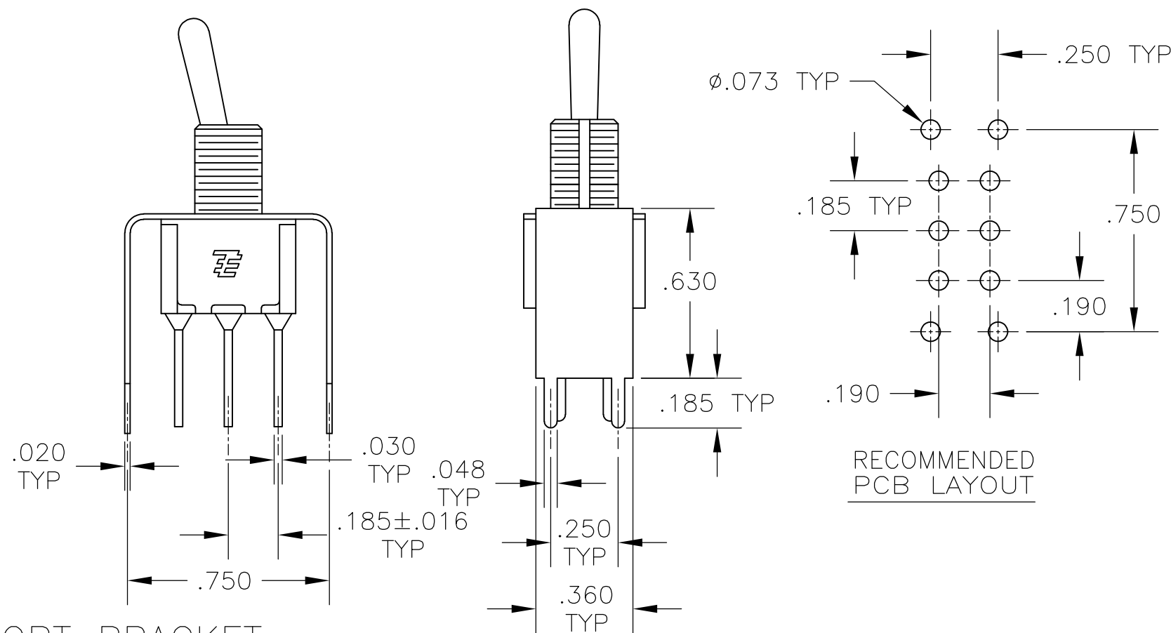
VERTICAL SUPPORT BRACKET
