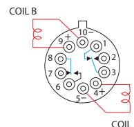
SCHEMATIC (Coil A Last Energized) 422H
