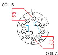
SCHEMATIC (Coil A Last Energized) (Bottom View)
