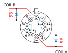
SCHEMATIC (Coil A Last Energized) (Bottom View)
