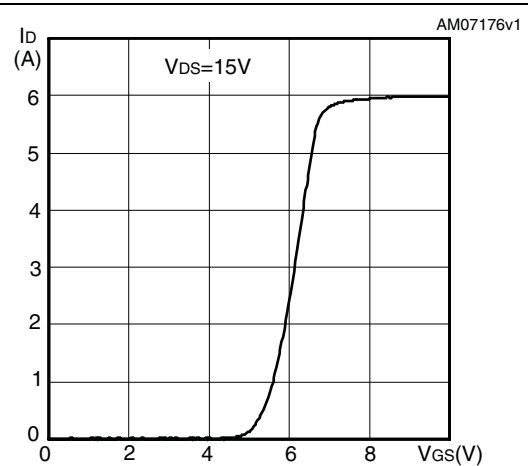
Figure 9. Transfer characteristics
