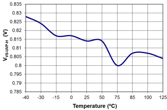
Figure 17. Output Under-Voltage Protection ( V_{S-UVP-H} ) vs. Temperature
