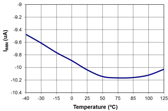
Figure 19. IMIN Pin Current ( I_{MIN} ) vs. Temperature
