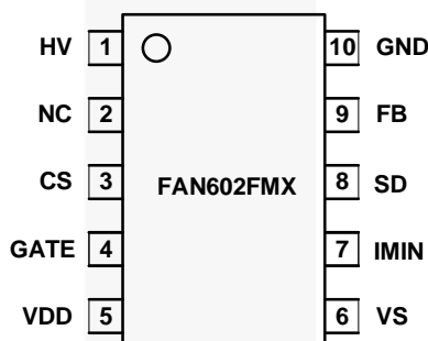
Figure 4. Pin Assignment
