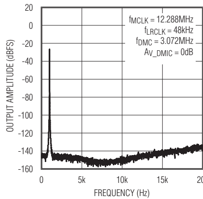
INBAND OUTPUT SPECTRUM, -26dBFS INPUT (DIGITAL MIC TO RECORD PATH)
