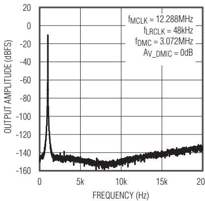
INBAND OUTPUT SPECTRUM, -10dBFS INPUT (DIGITAL MIC TO RECORD PATH)
