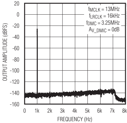
INBAND OUTPUT SPECTRUM, -26dBFS INPUT (DIGITAL MIC TO RECORD PATH)
