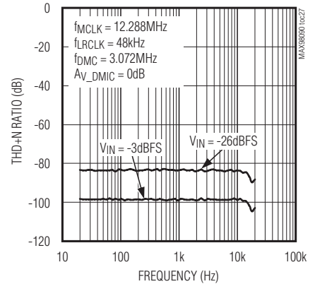
TOTAL HARMONIC DISTORTION PLUS NOISE vs. FREQUENCY (DIGITAL MIC TO RECORD PATH)
