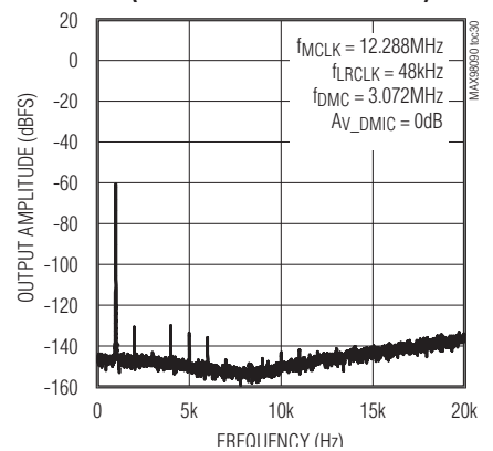
INBAND OUTPUT SPECTRUM, -60dBFS INPUT (DIGITAL MIC TO RECORD PATH)
