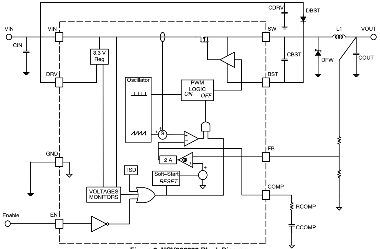
Figure 2. NCV890230 Block Diagram
