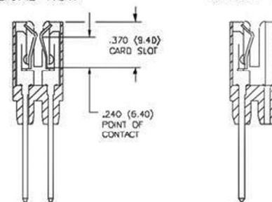
FOR IN-CONTACT POLARIZING USE KEY P/N 321-240-328 FOR BETWEEN CONTACT POLARIZING USE KEY P/N 243-240-318
