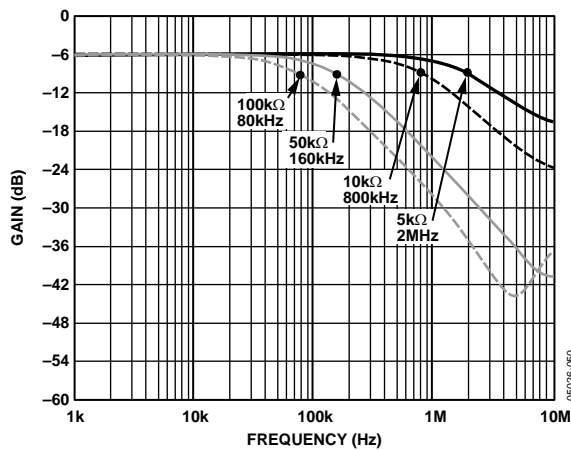
Figure 26. -3\text{ dB} Bandwidth @ Code = 0x80
