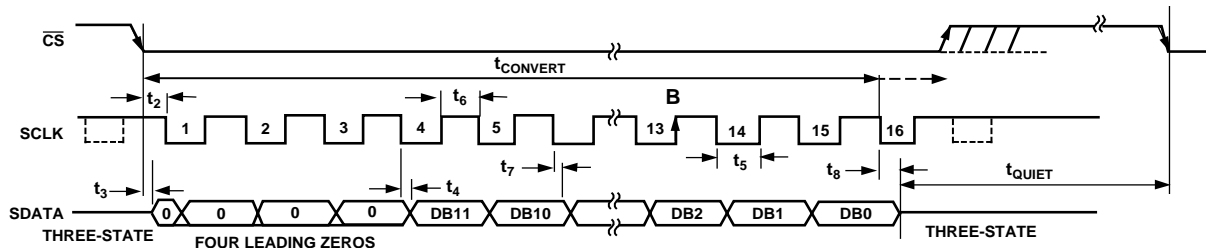
Figure 26. Serial Interface Timing Diagram
