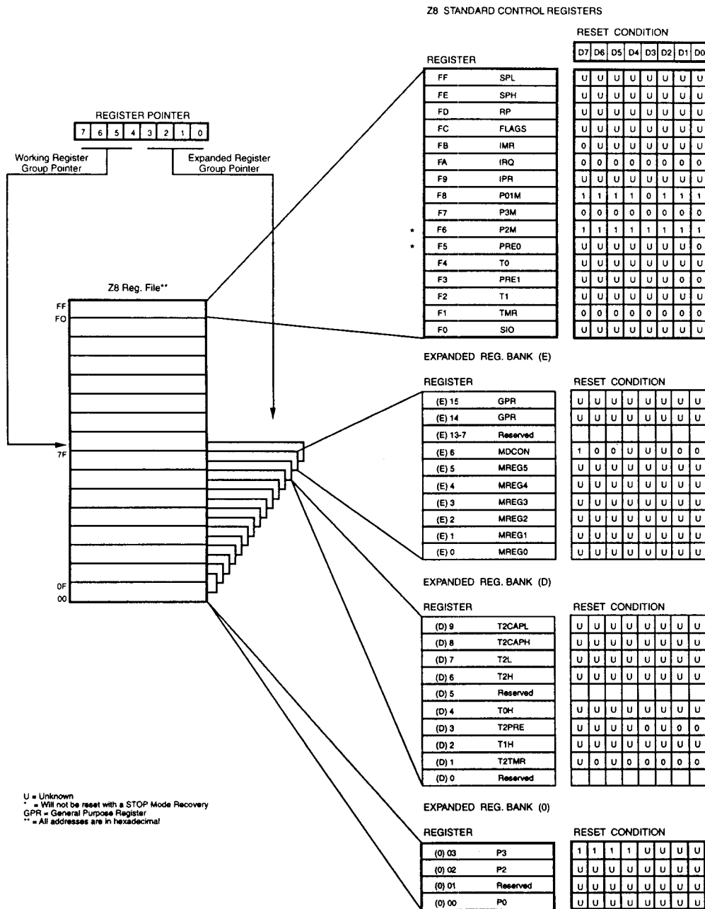
Figure 13. Register File
