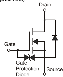
Equivalent Circuit
