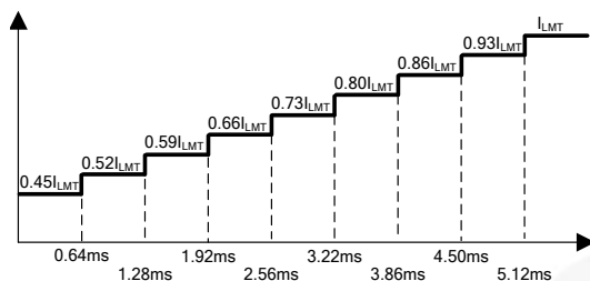
Figure 22. Current Limit Variation During Soft-Start
