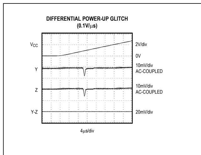
Figure 7. Differential Power-Up Glitch (0.1V/μs)
