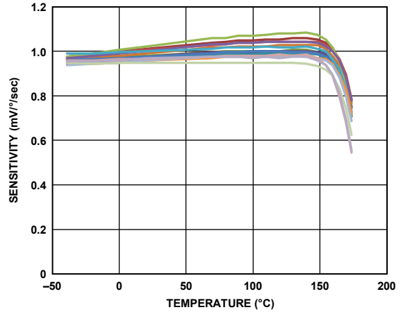
Figure 9. Sensitivity Over Temperature
