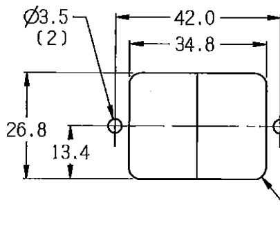
PANEL CUTOUT FRONT MOUNT TOLERANCE \pm .13
