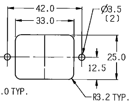
PANEL CUTOUT REAR MOUNT TOLERANCE \pm .13
