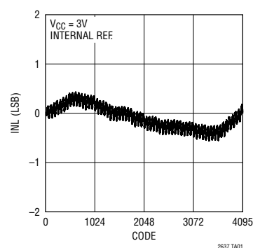
Integral Nonlinearity (LTC2637-LZ12)
