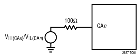
Test Circuit 1
