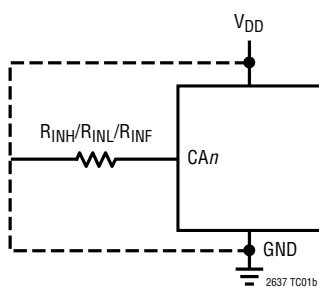
Test Circuit 2
