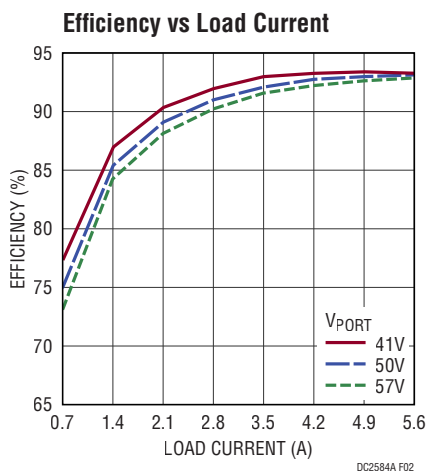
Figure 2. Efficiency (End-to-End)
