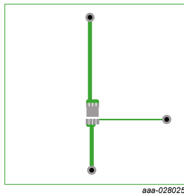
70 μm copper; FR4 Board
