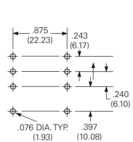
2 pole version
