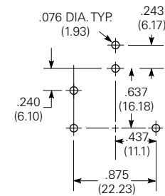
1 pole version
