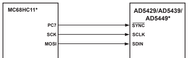
Figure 53. MCH68HC11/68L11-to-AD5429/AD5439/AD5449 Interface
