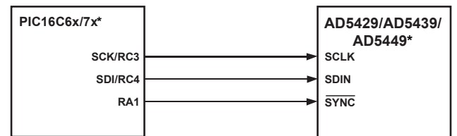
Figure 55. PIC16C6x/7x-to-AD5429/AD5439/AD5449 Interface
