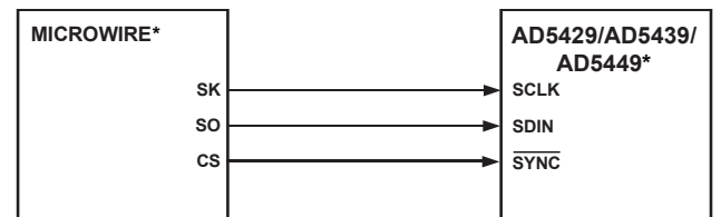
Figure 54. MICROWIRE-to-AD5429/AD5439/AD5449 Interface
