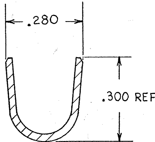
SECTION C-C
