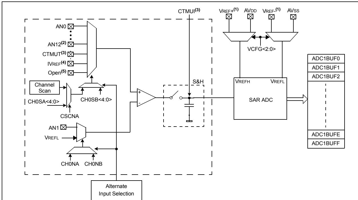
FIGURE 22-1: ADC1 MODULE BLOCK DIAGRAM
