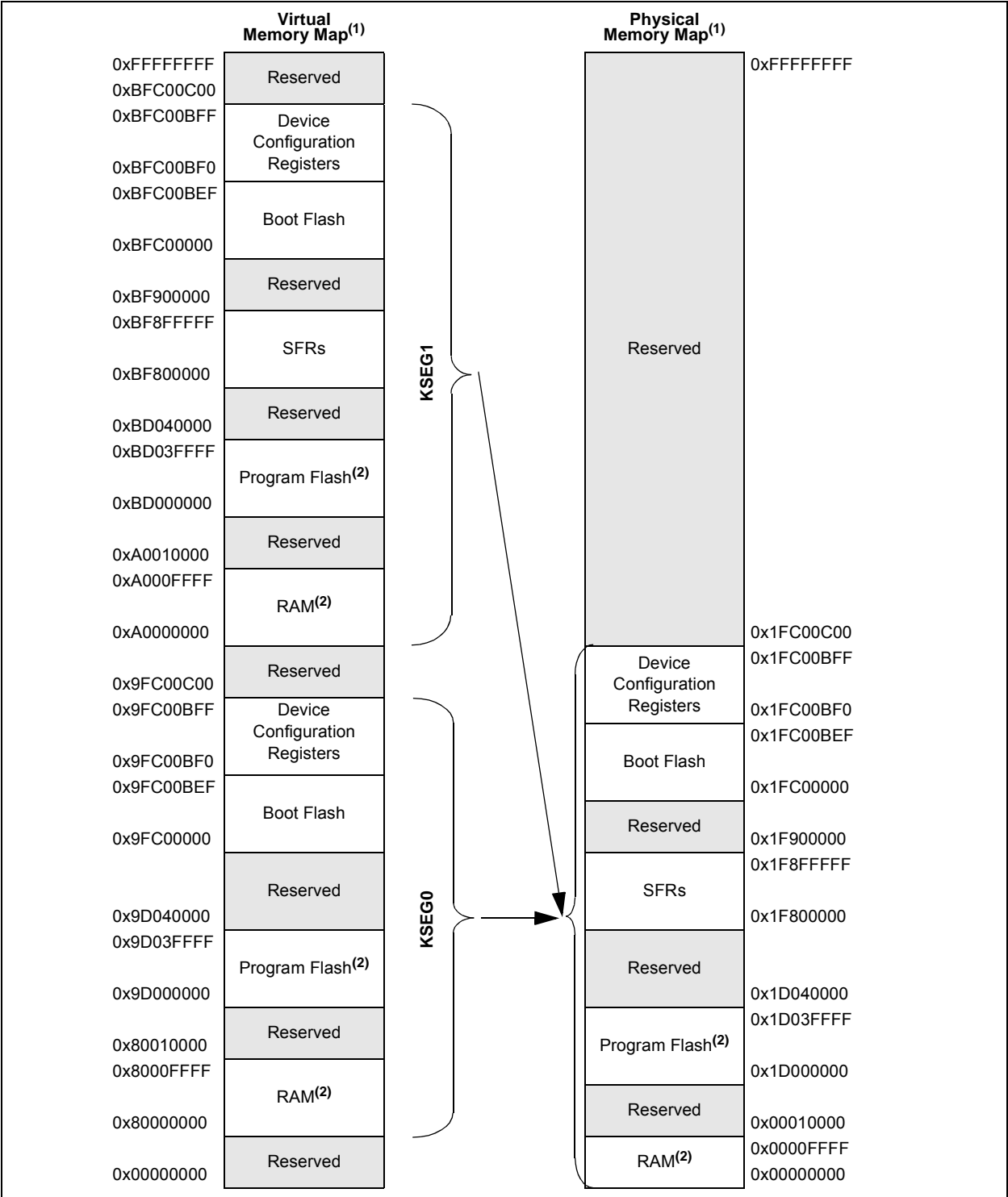
FIGURE 4-5: MEMORY MAP ON RESET FOR PIC32MX170/270 DEVICES (64 KB RAM, 256 KB FLASH)
