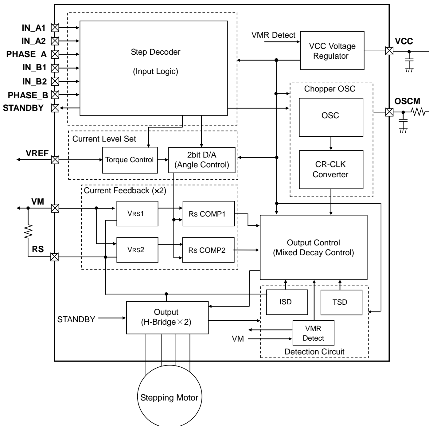
Block Diagram
