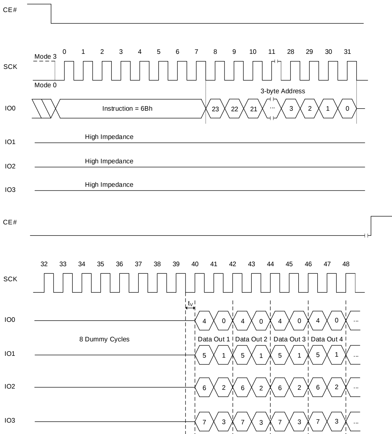
Figure 8.6 Fast Read Quad-Output Sequence
