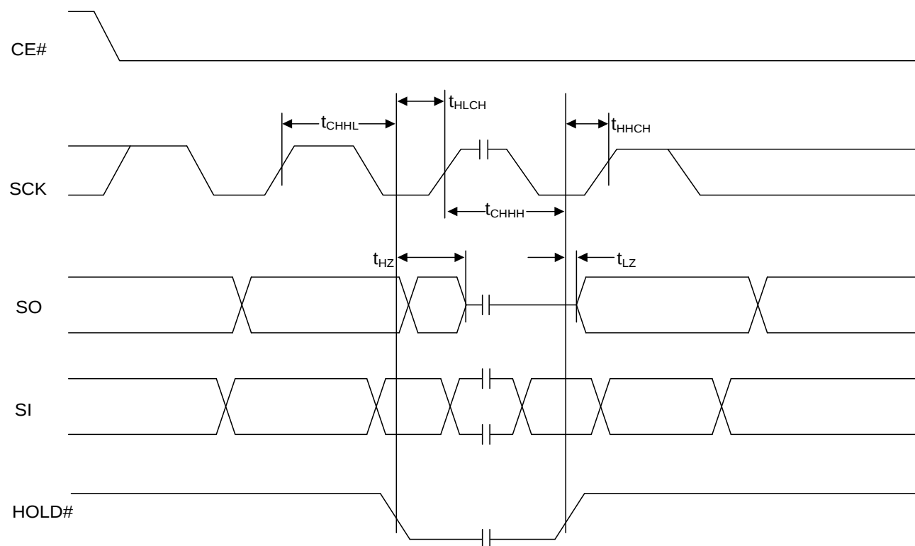
Figure 9.3 HOLD TIMING
