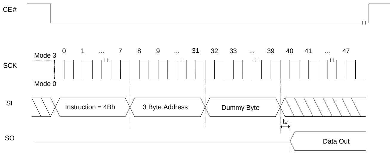
Figure 8.25 RDUID Operation
