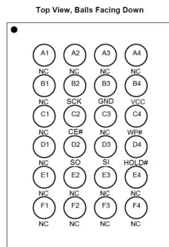
TFBGA-24 6x8mm (Package: JG)
