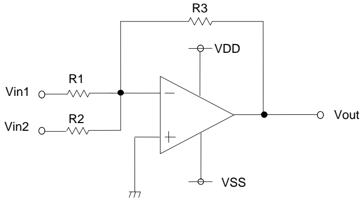
Fig. 193 Adder circuit
