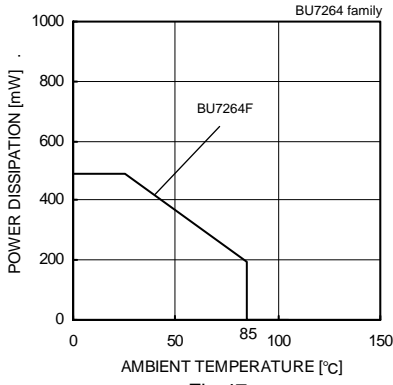
Fig.47 Derating curve
